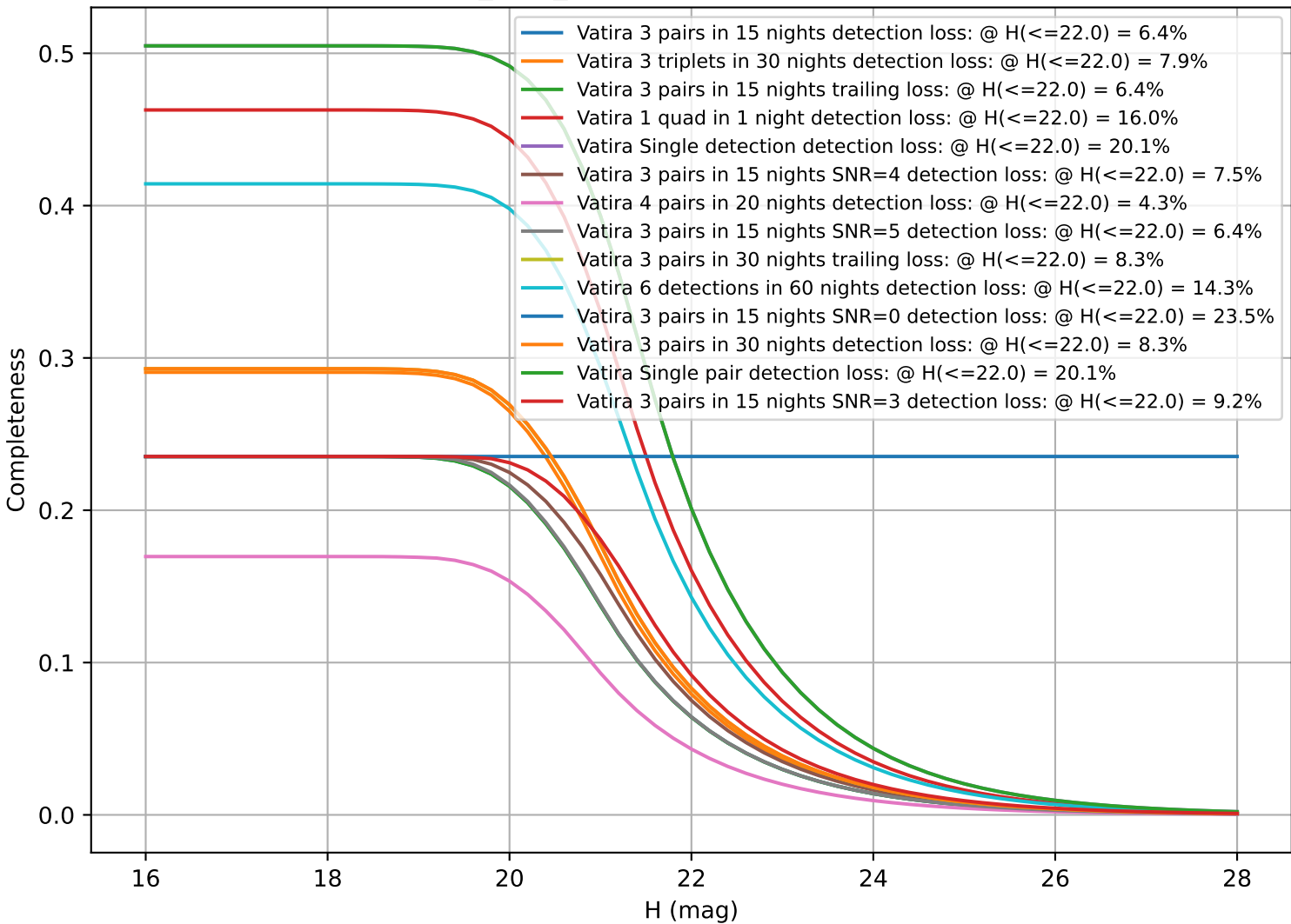
baseline_v3.2_10yrs: CumulativeCompleteness
