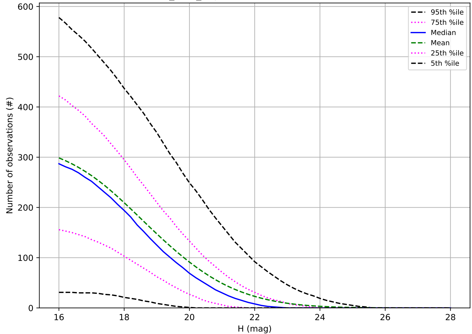
baseline_v3.2_10yrs: Number of observations NEO
