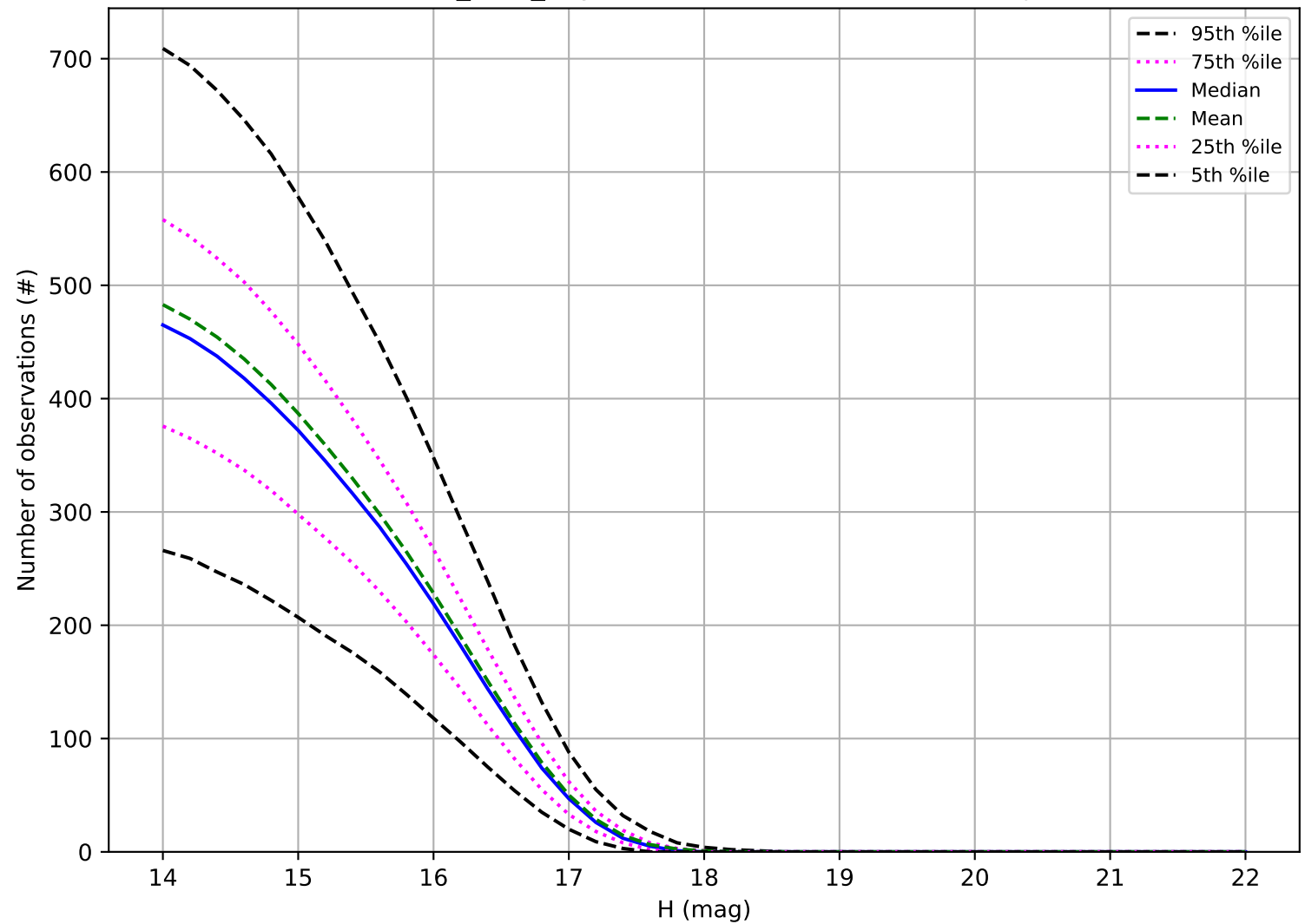
baseline_v3.2_10yrs: Number of observations Trojan
