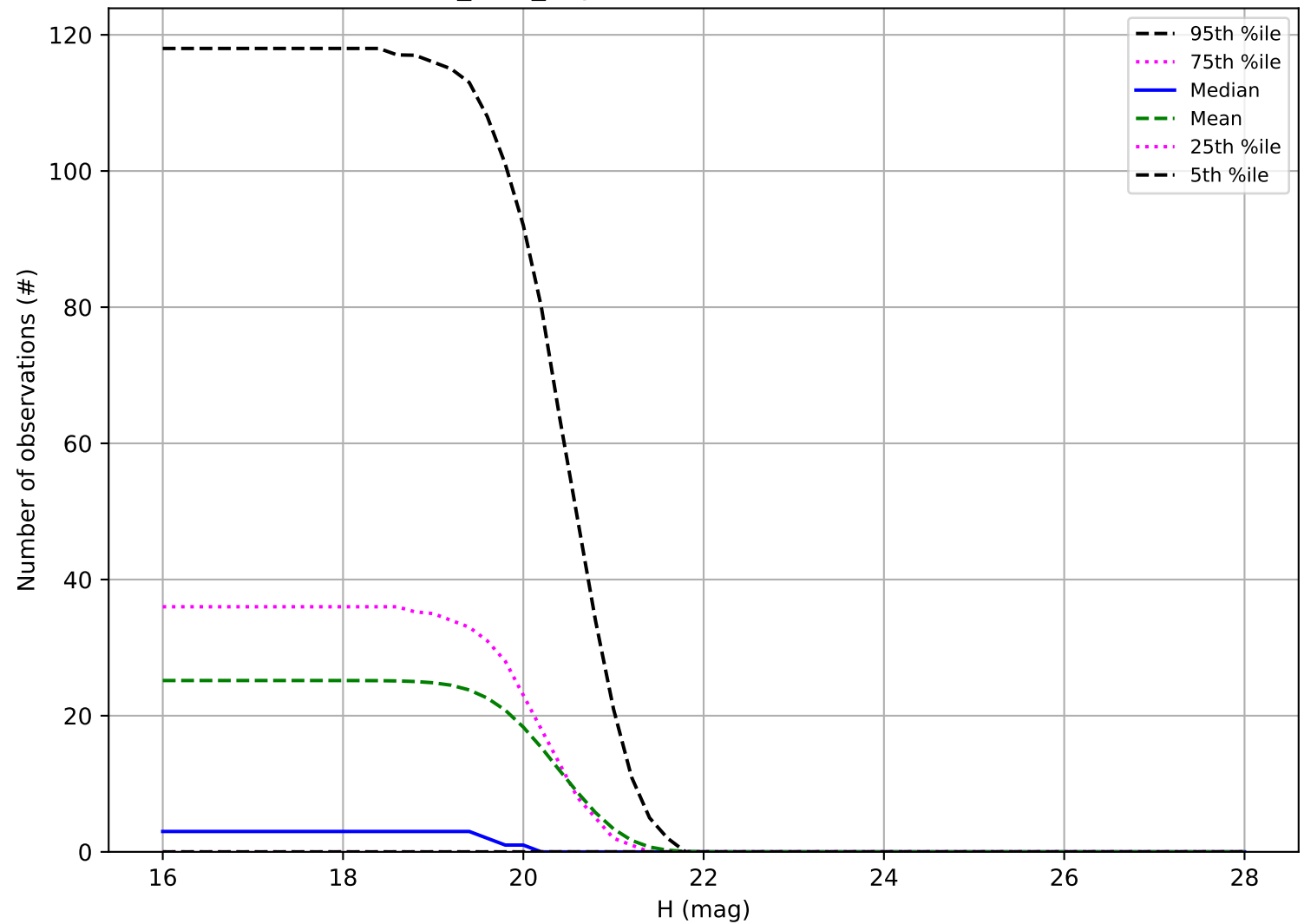
baseline_v3.2_10yrs: Number of observations Vatira
