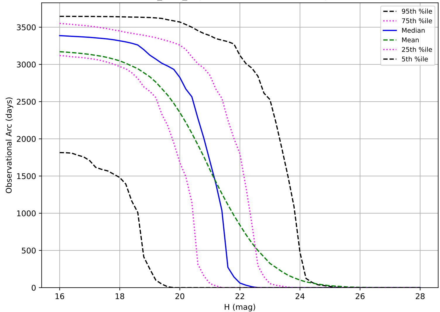
baseline_v3.2_10yrs: Observational Arc Length NEO
