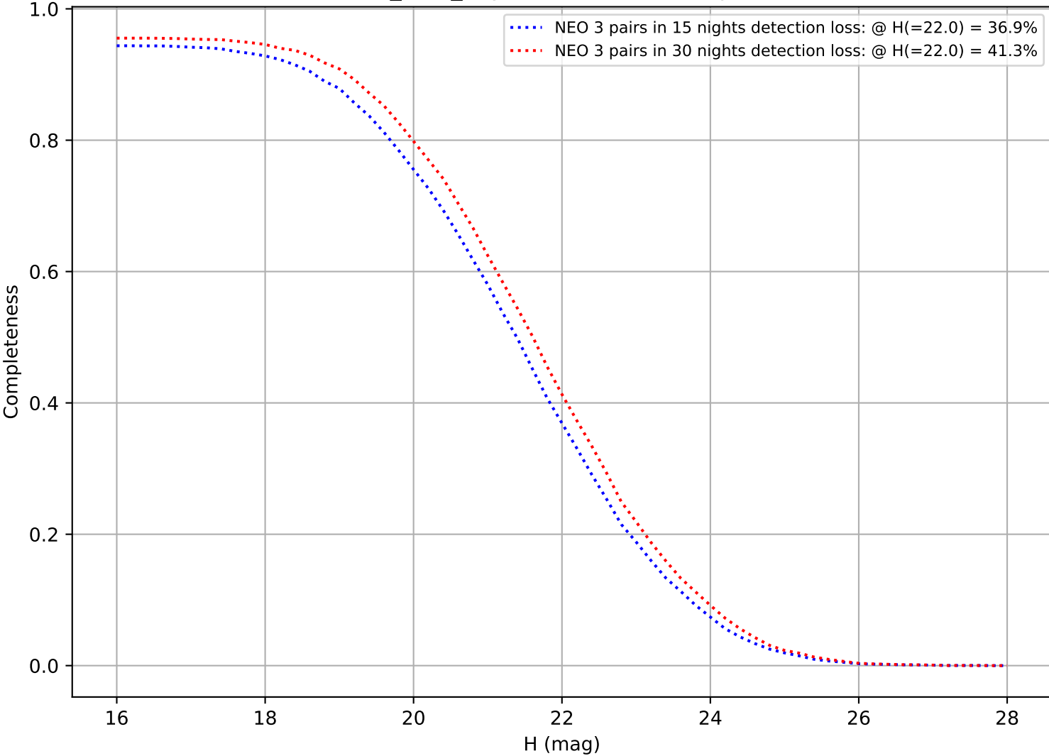
baseline_v3.3_10yrs: DifferentialCompleteness
