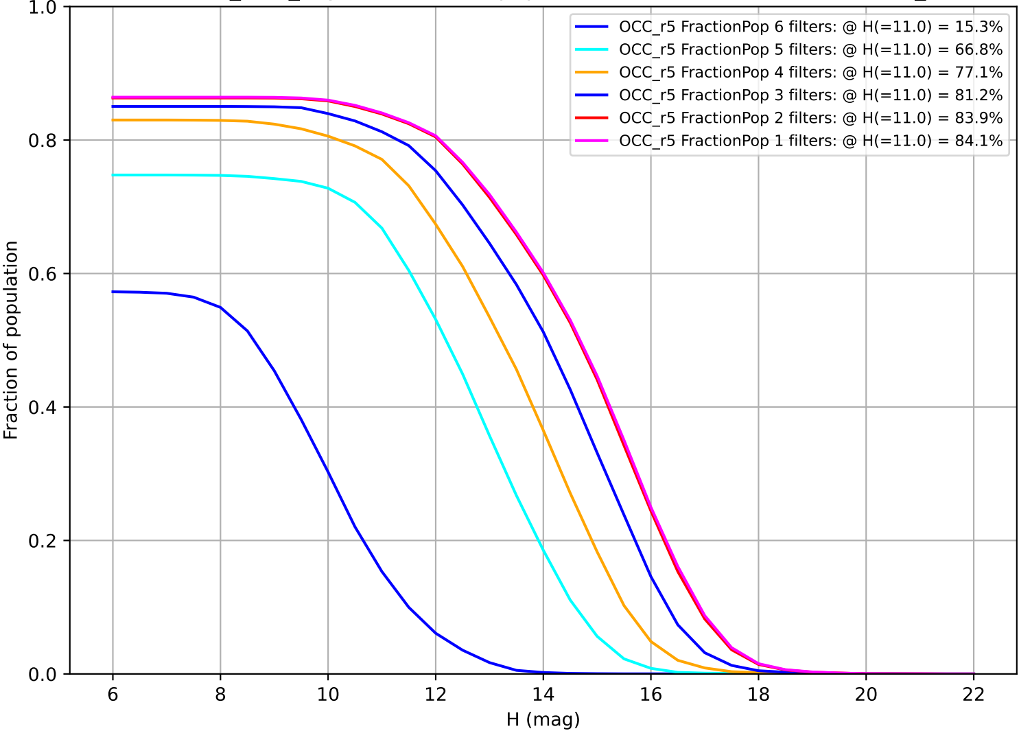
baseline_v3.3_10yrs: Fraction of population with colors in X filters OCC_r5
