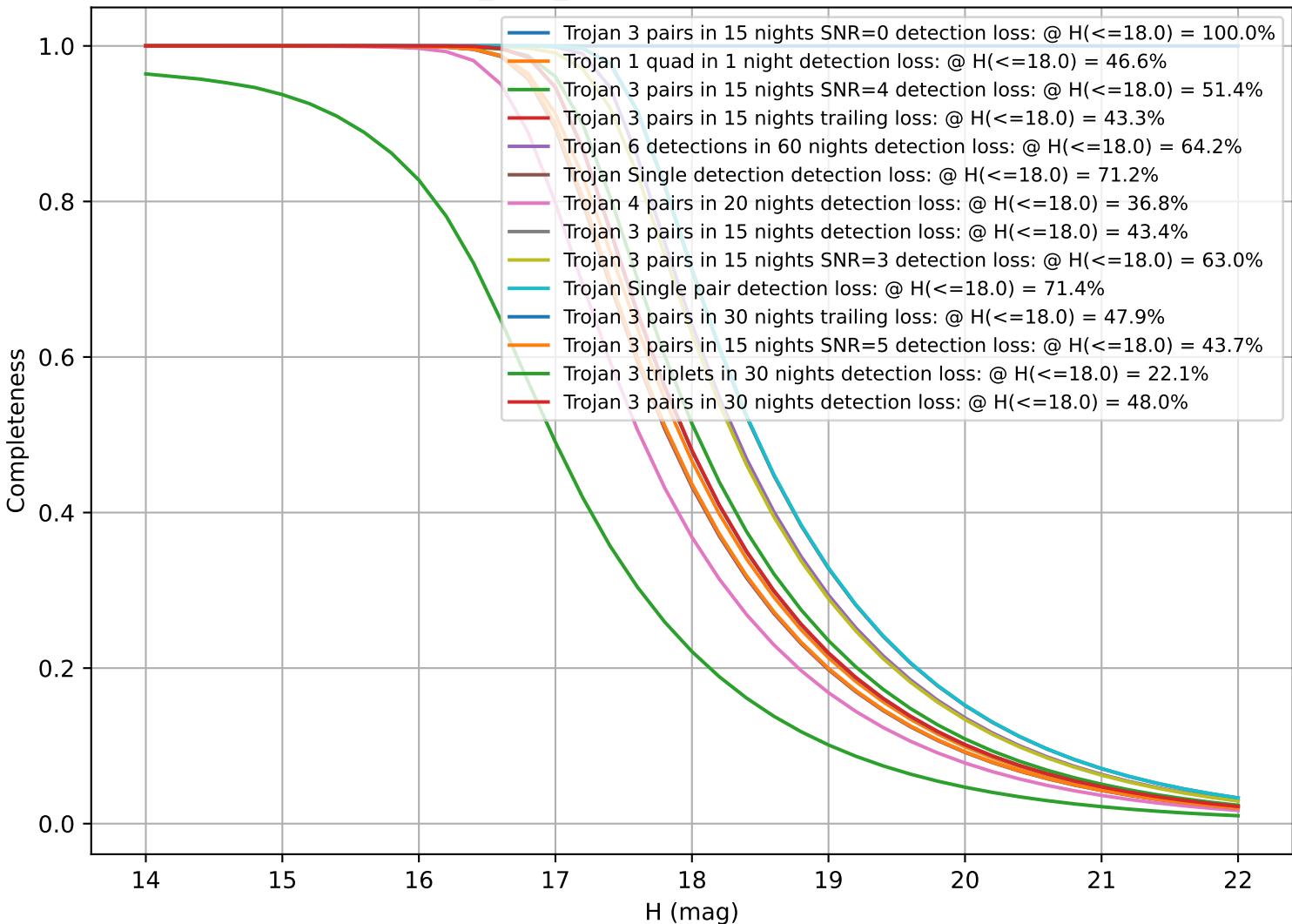
baseline_v3.3_10yrs: CumulativeCompleteness
