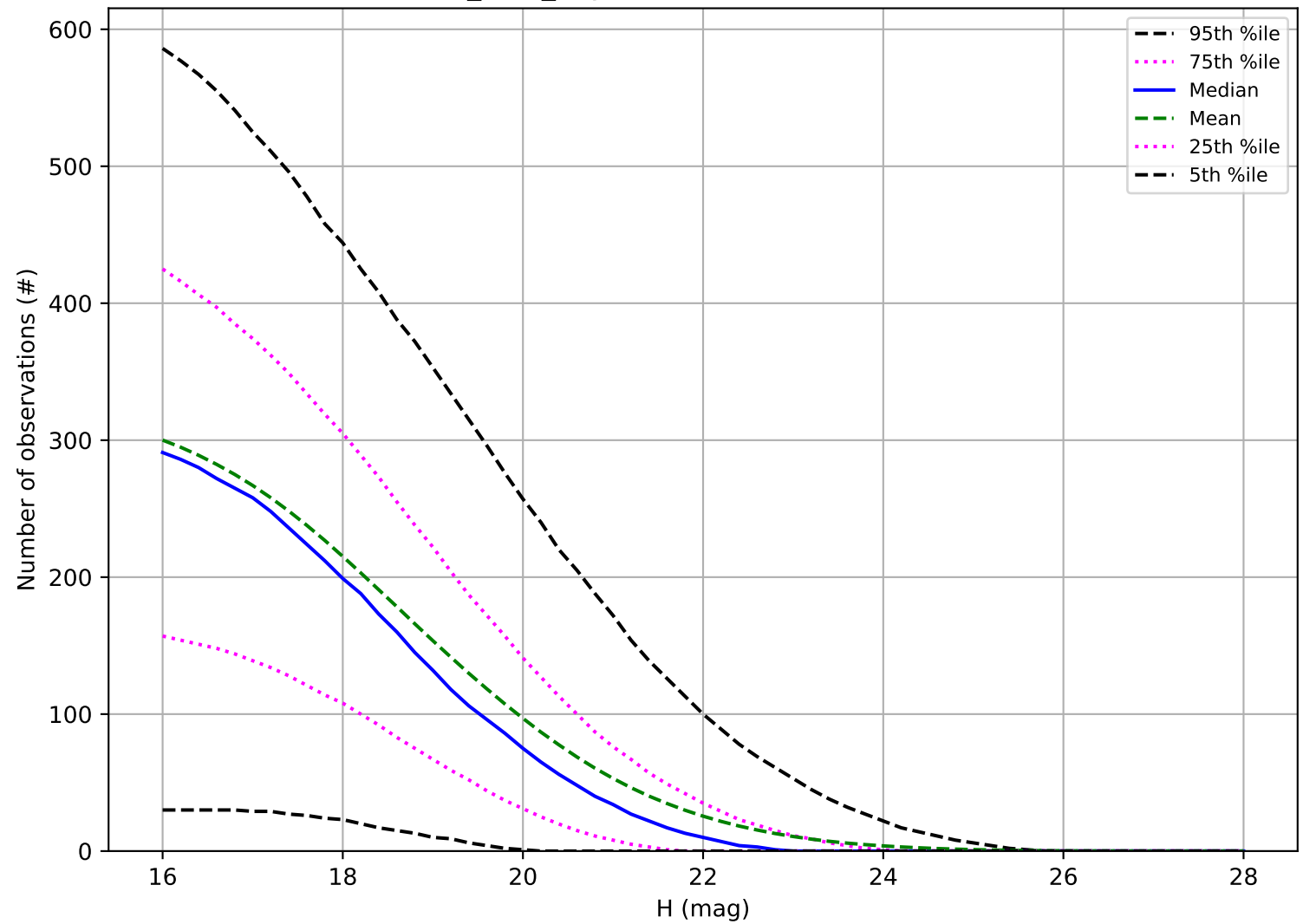
baseline_v3.3_10yrs: Number of observations NEO
