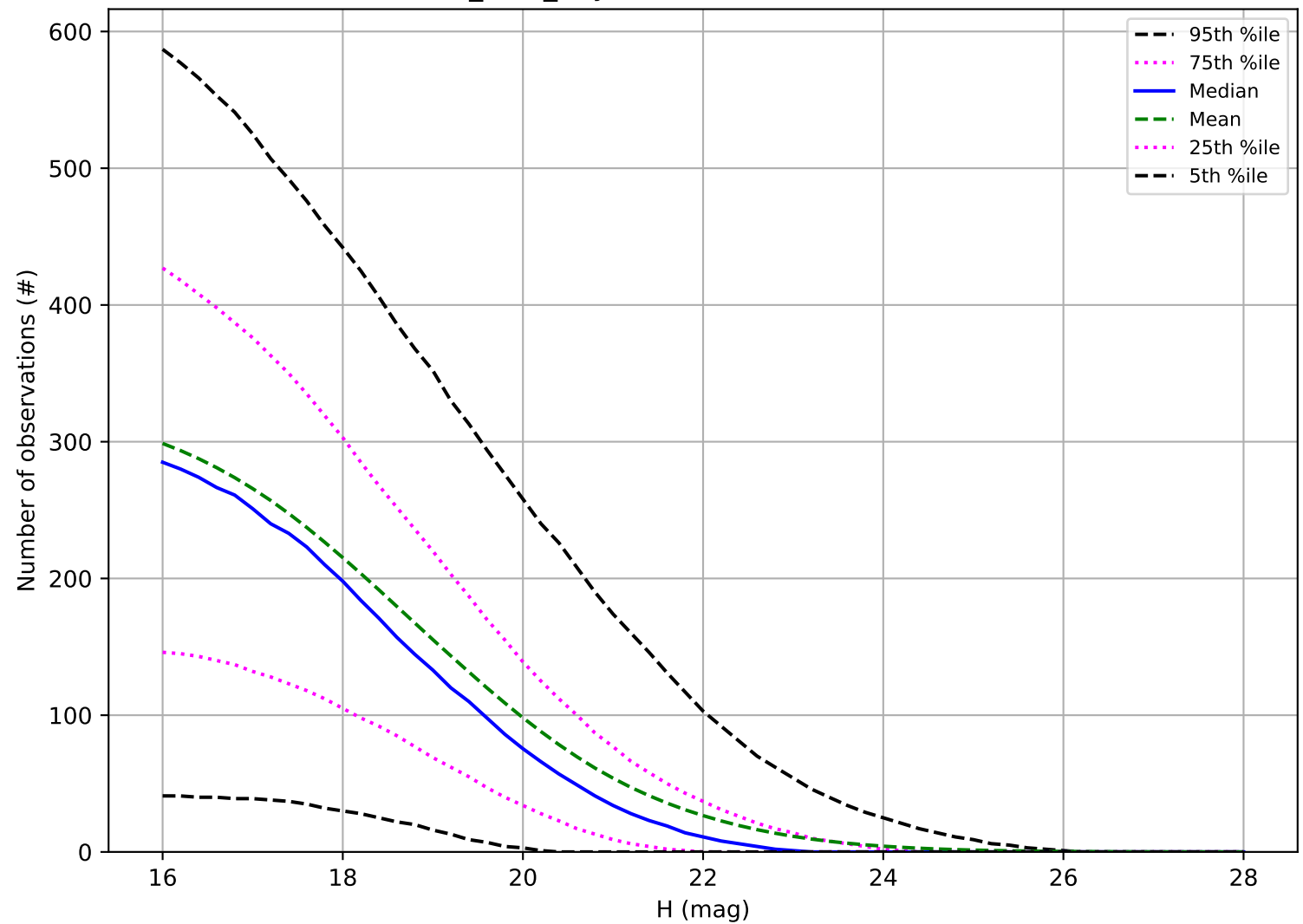
baseline_v3.3_10yrs: Number of observations PHA
