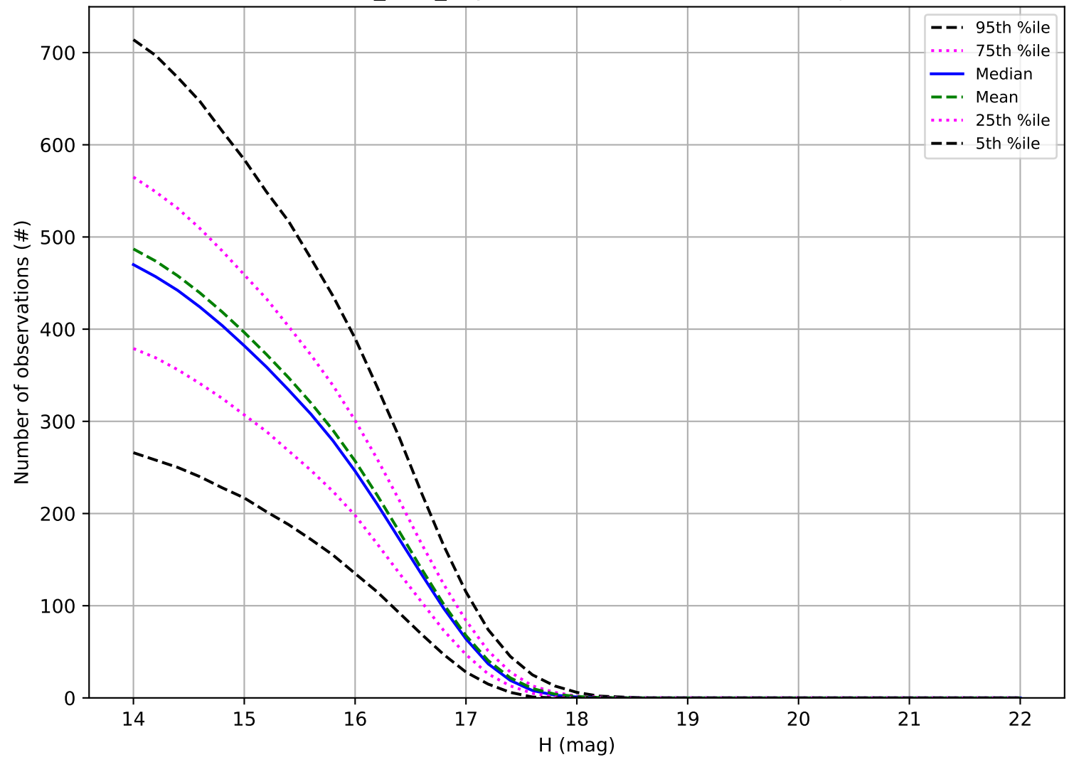
baseline_v3.3_10yrs: Number of observations Trojan
