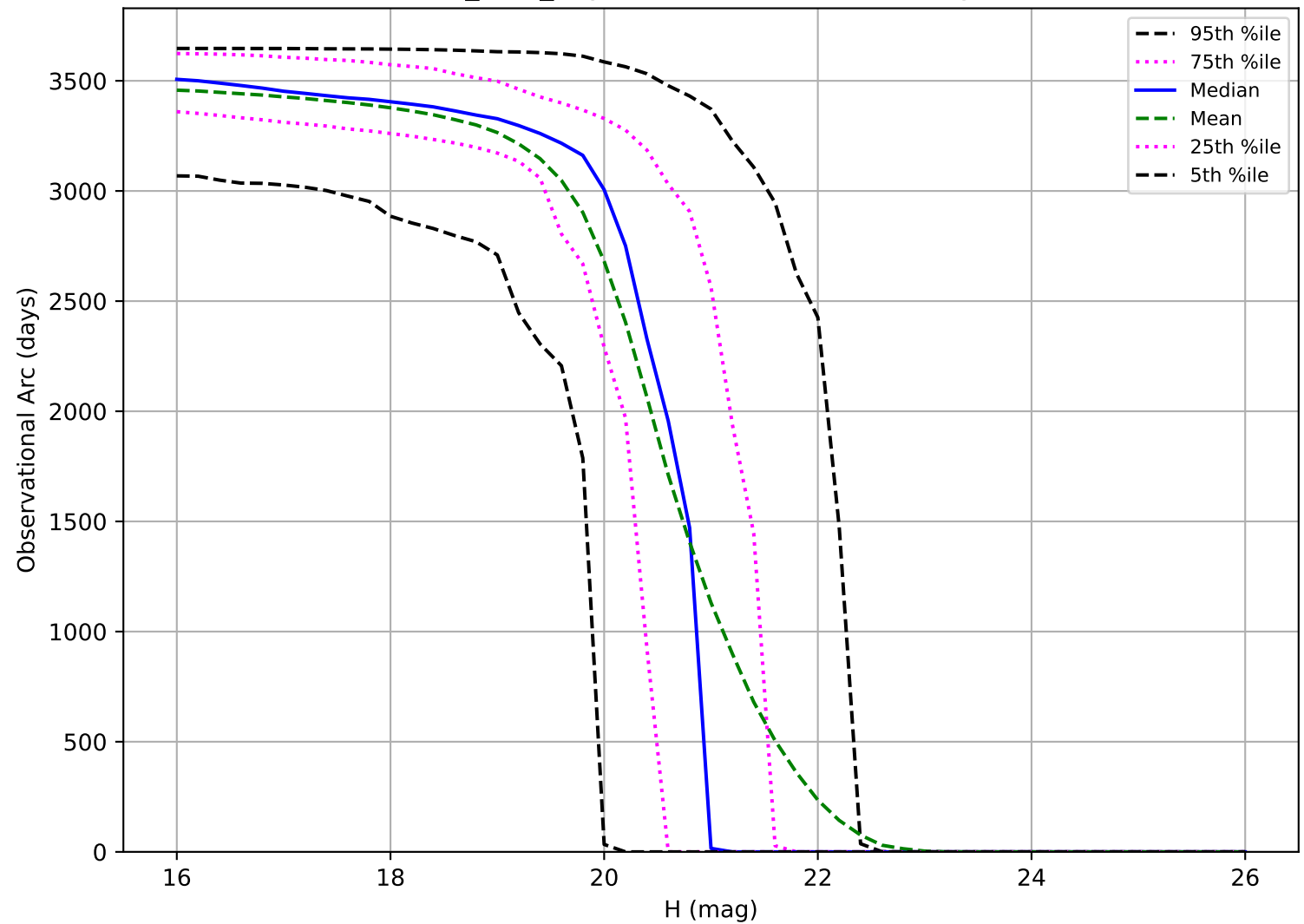
baseline_v3.3_10yrs: Observational Arc Length MBA
