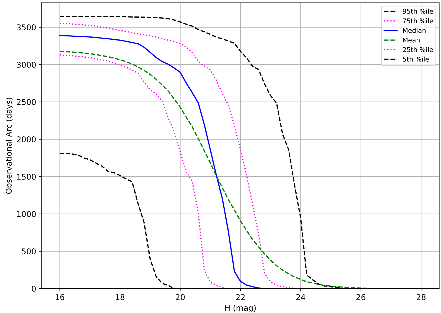
baseline_v3.3_10yrs: Observational Arc Length NEO
