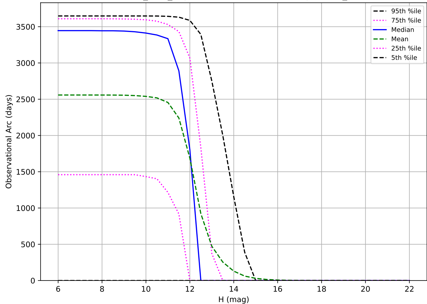
baseline_v3.3_10yrs: Observational Arc Length OCC_r20
