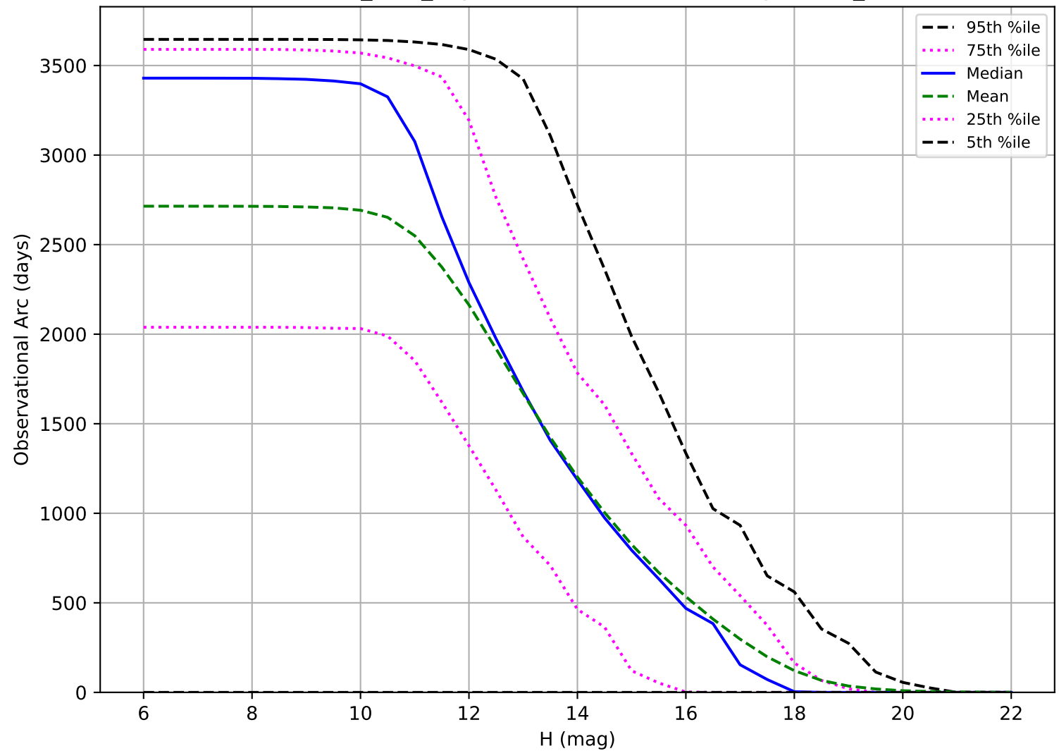
baseline_v3.3_10yrs: Observational Arc Length OCC_r5
