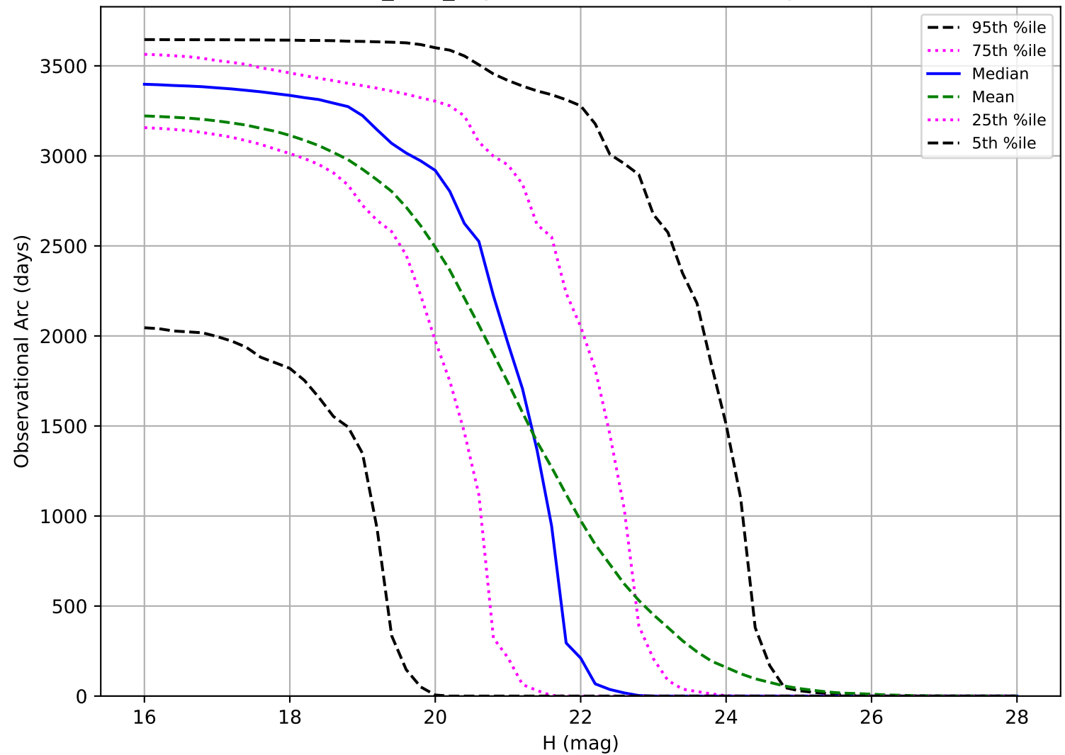
baseline_v3.3_10yrs: Observational Arc Length PHA
