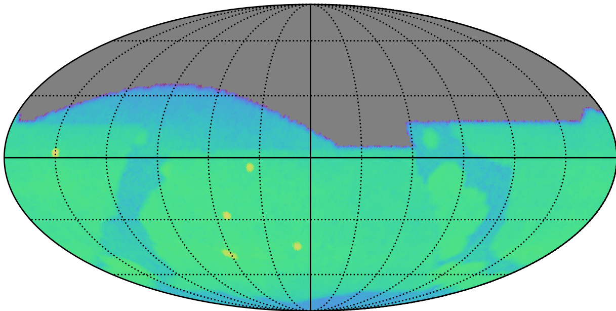
baseline_v3.4_10yrs g: CoaddM5
