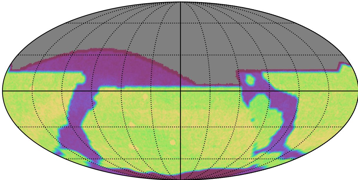
baseline_v3.4_10yrs : Count observationStartMJD
