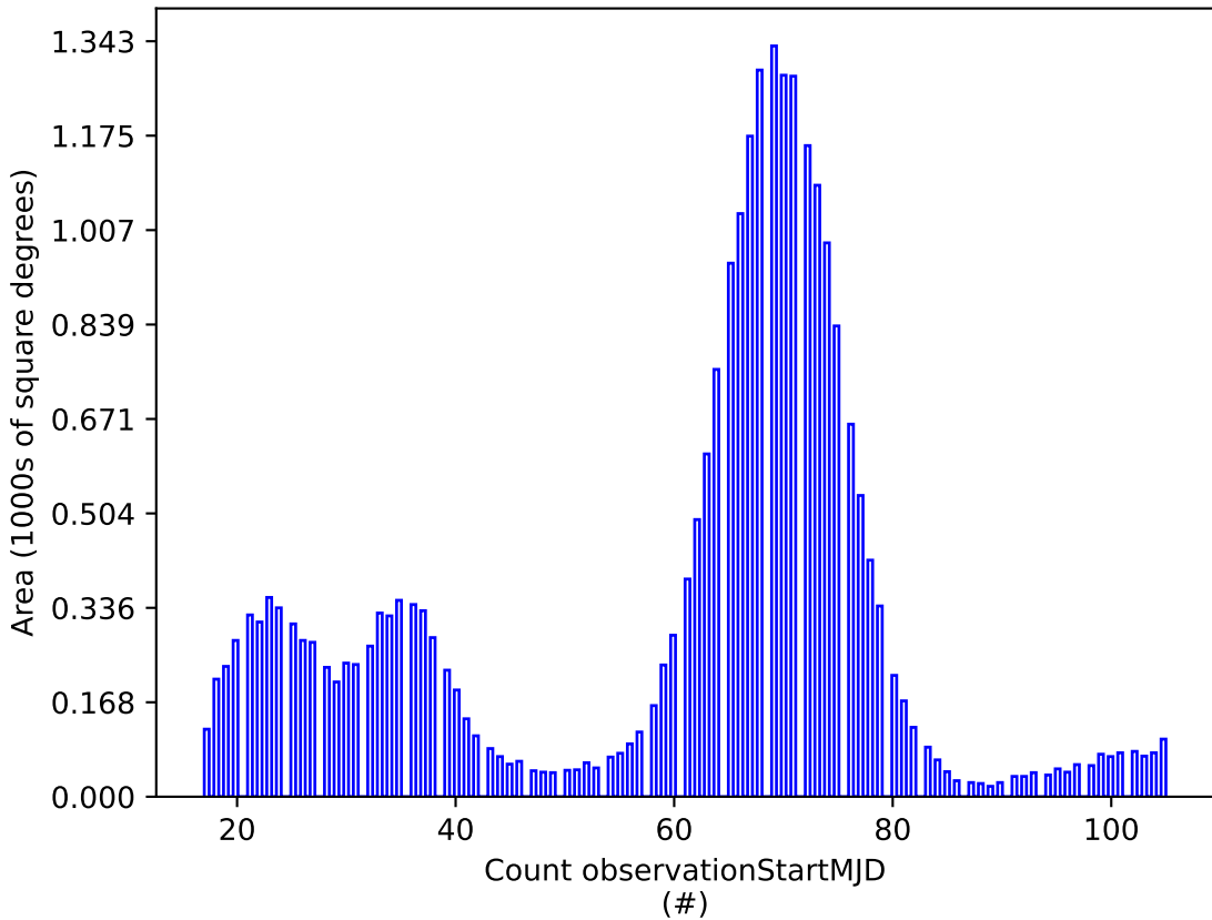
baseline_v3.4_10yrs g: Count observationStartMJD
