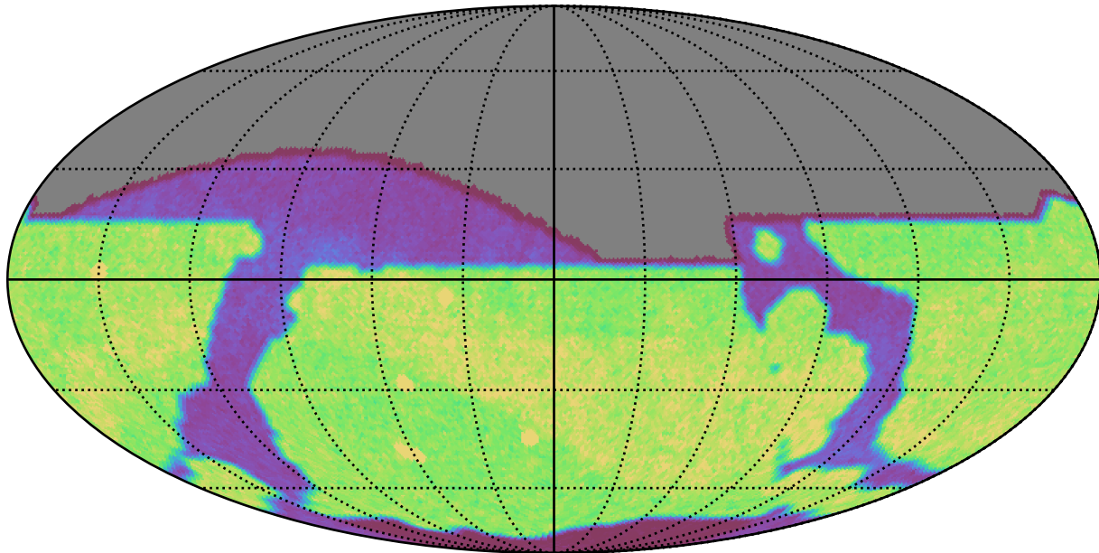
baseline_v3.4_10yrs i: Count observationStartMJD
