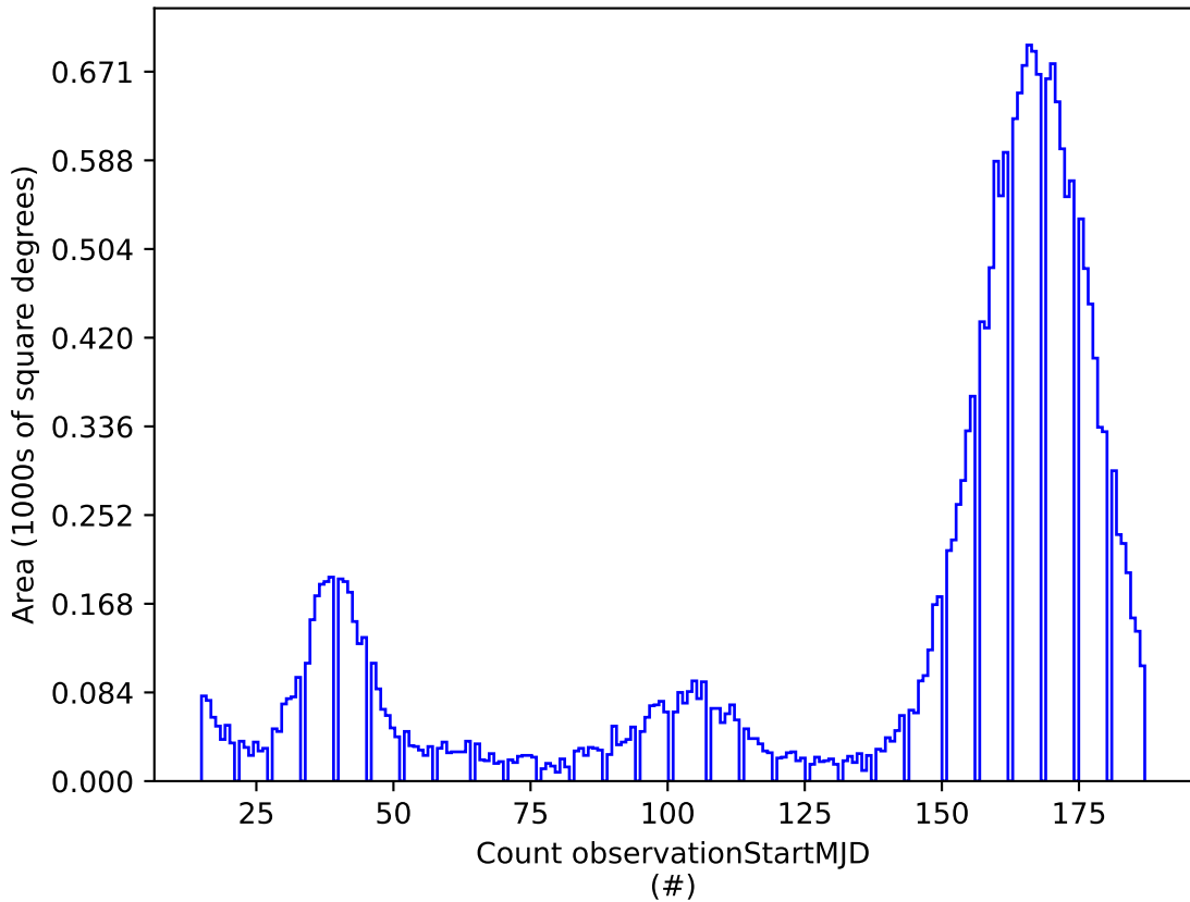
baseline_v3.4_10yrs y: Count observationStartMJD
