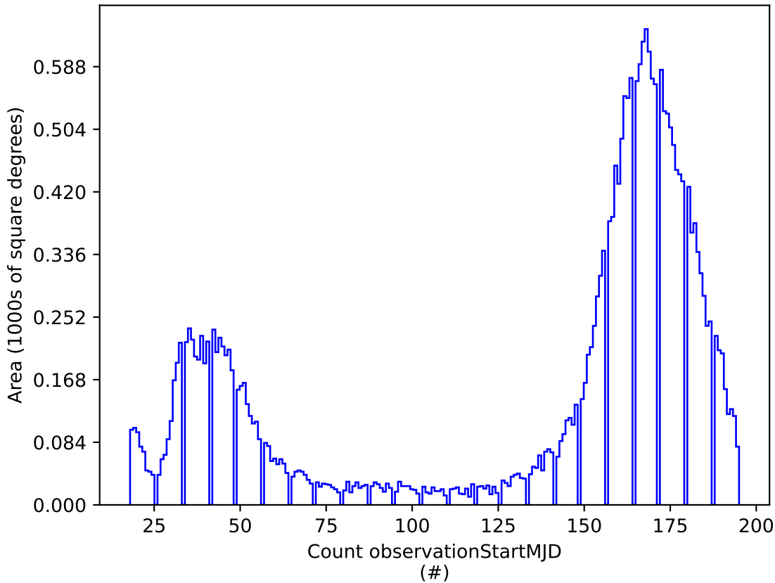
baseline_v3.4_10yrs z: Count observationStartMJD
