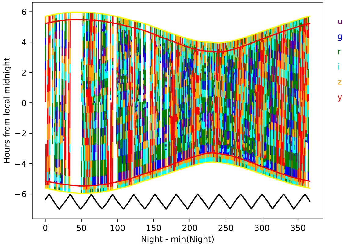
baseline_v3.4_10yrs year 6-7: Hourglass
