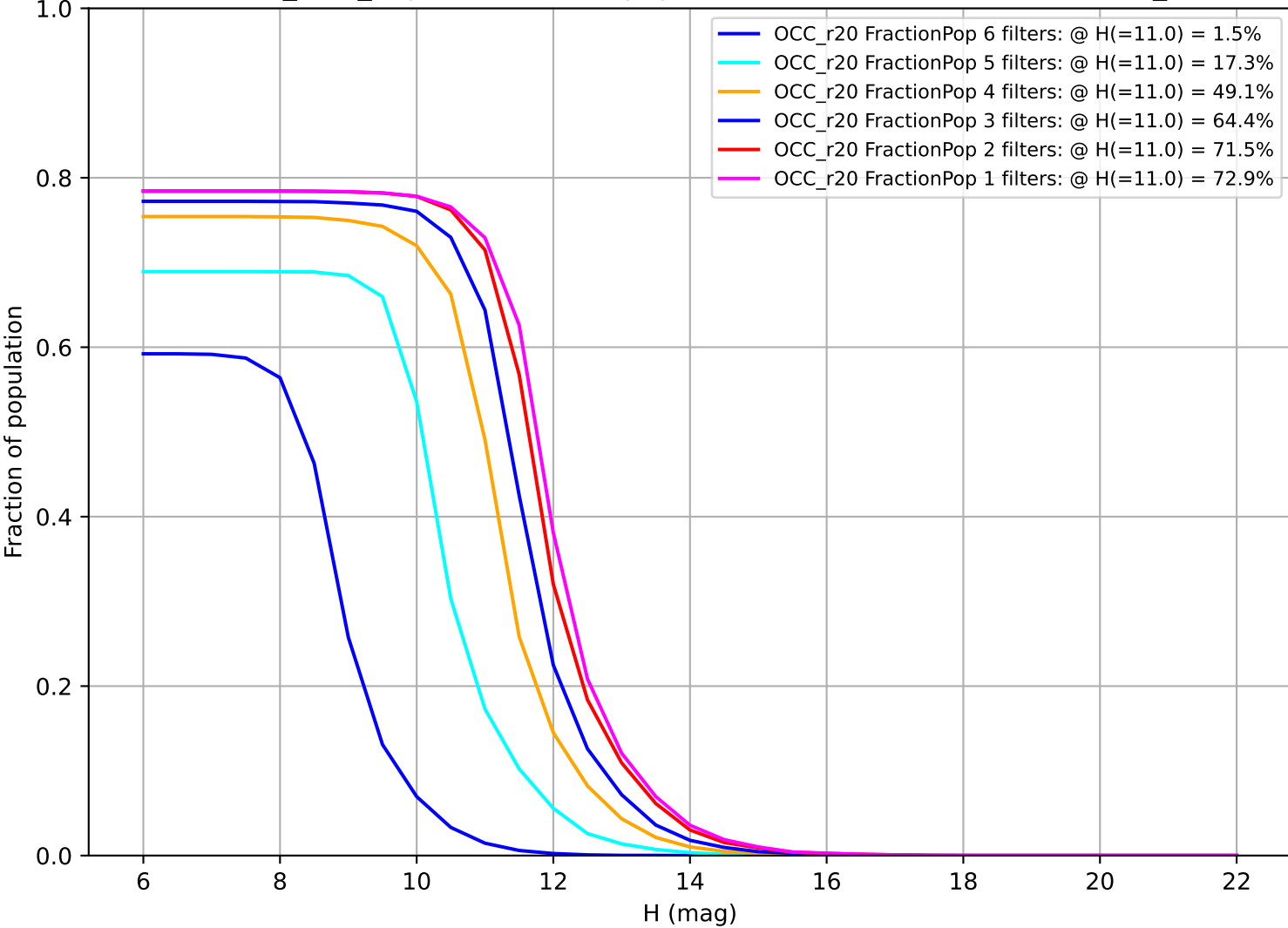
baseline_v3.4_10yrs: Fraction of population with colors in X filters OCC_r20
