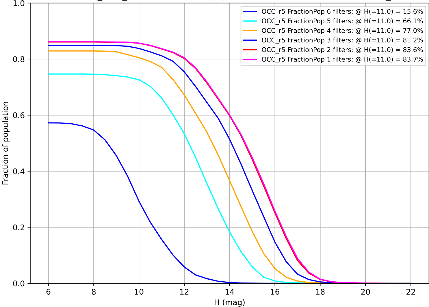
baseline_v3.4_10yrs: Fraction of population with colors in X filters OCC_r5
