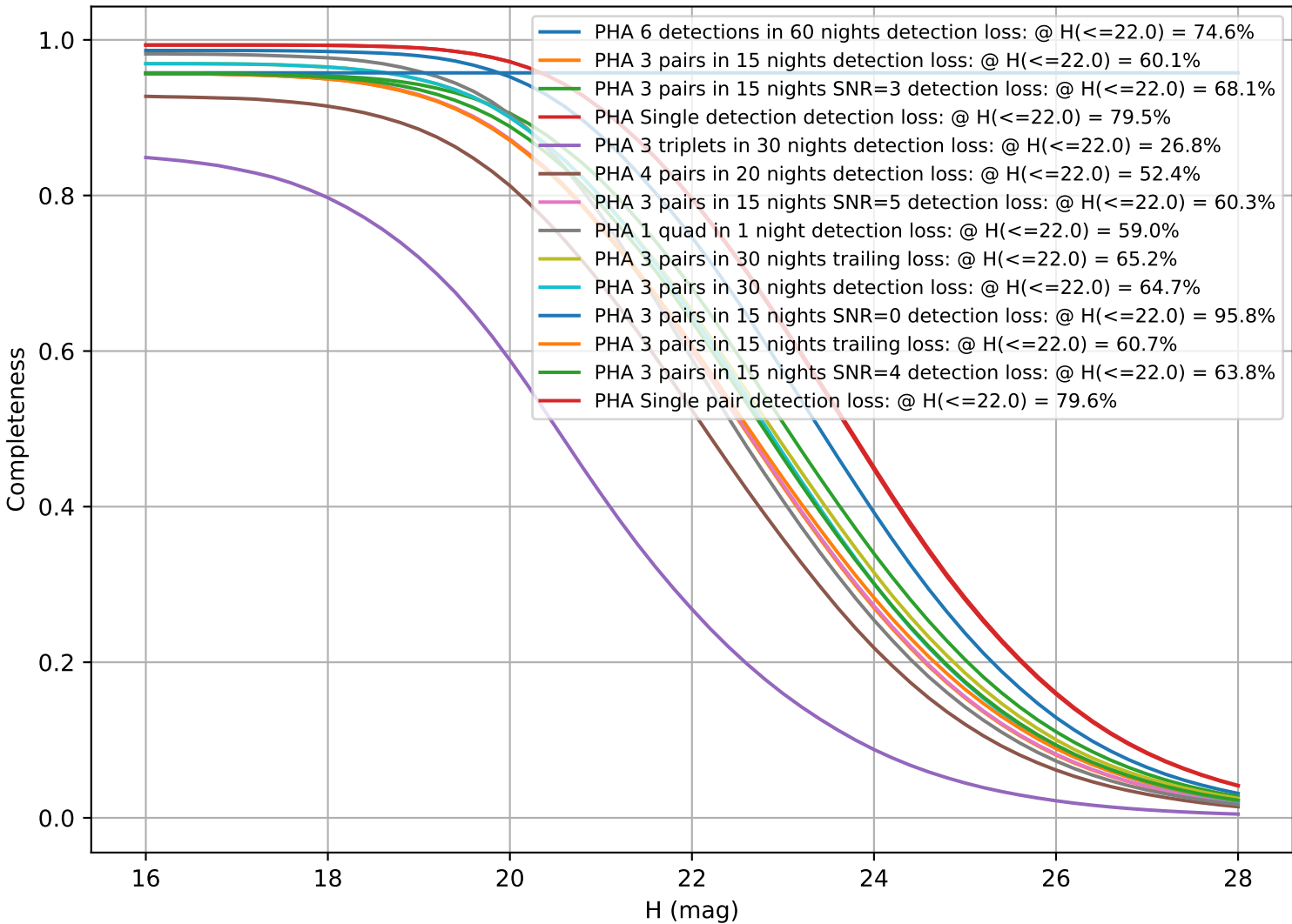
baseline_v3.4_10yrs: CumulativeCompleteness
