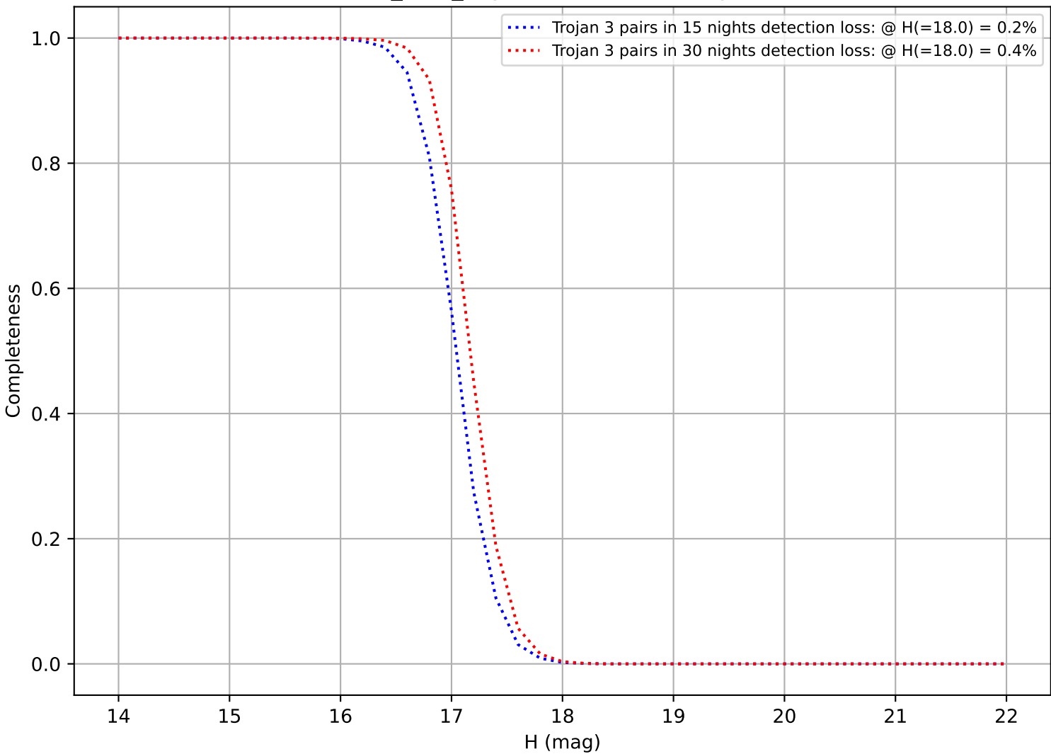
baseline_v3.4_10yrs: DifferentialCompleteness
