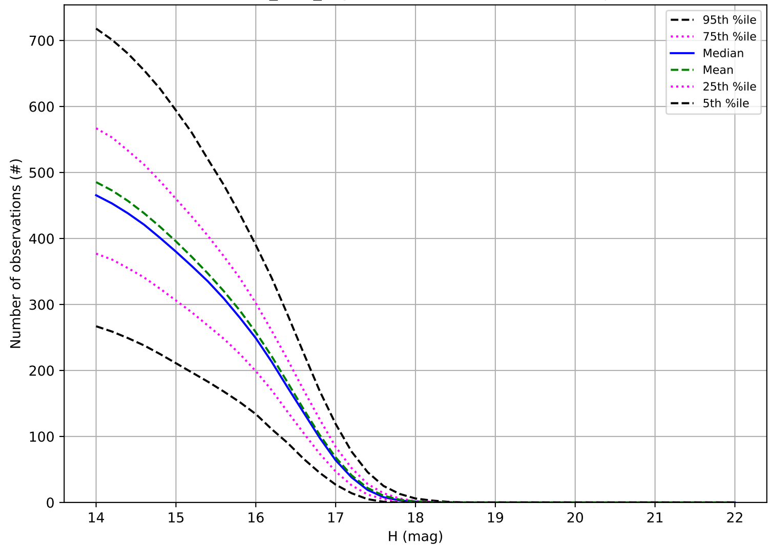
baseline_v3.4_10yrs: Number of observations Trojan
