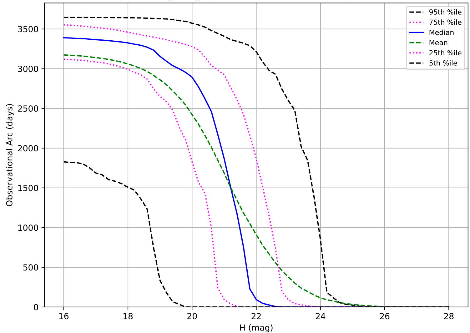
baseline_v3.4_10yrs: Observational Arc Length NEO
