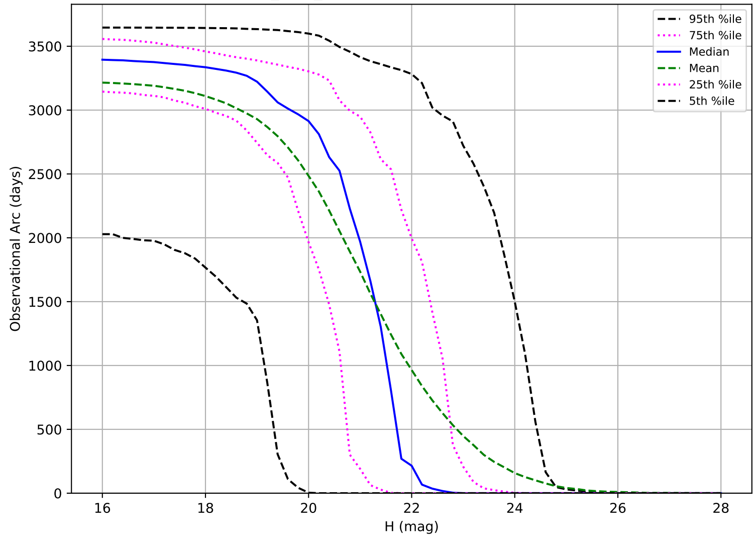
baseline_v3.4_10yrs: Observational Arc Length PHA
