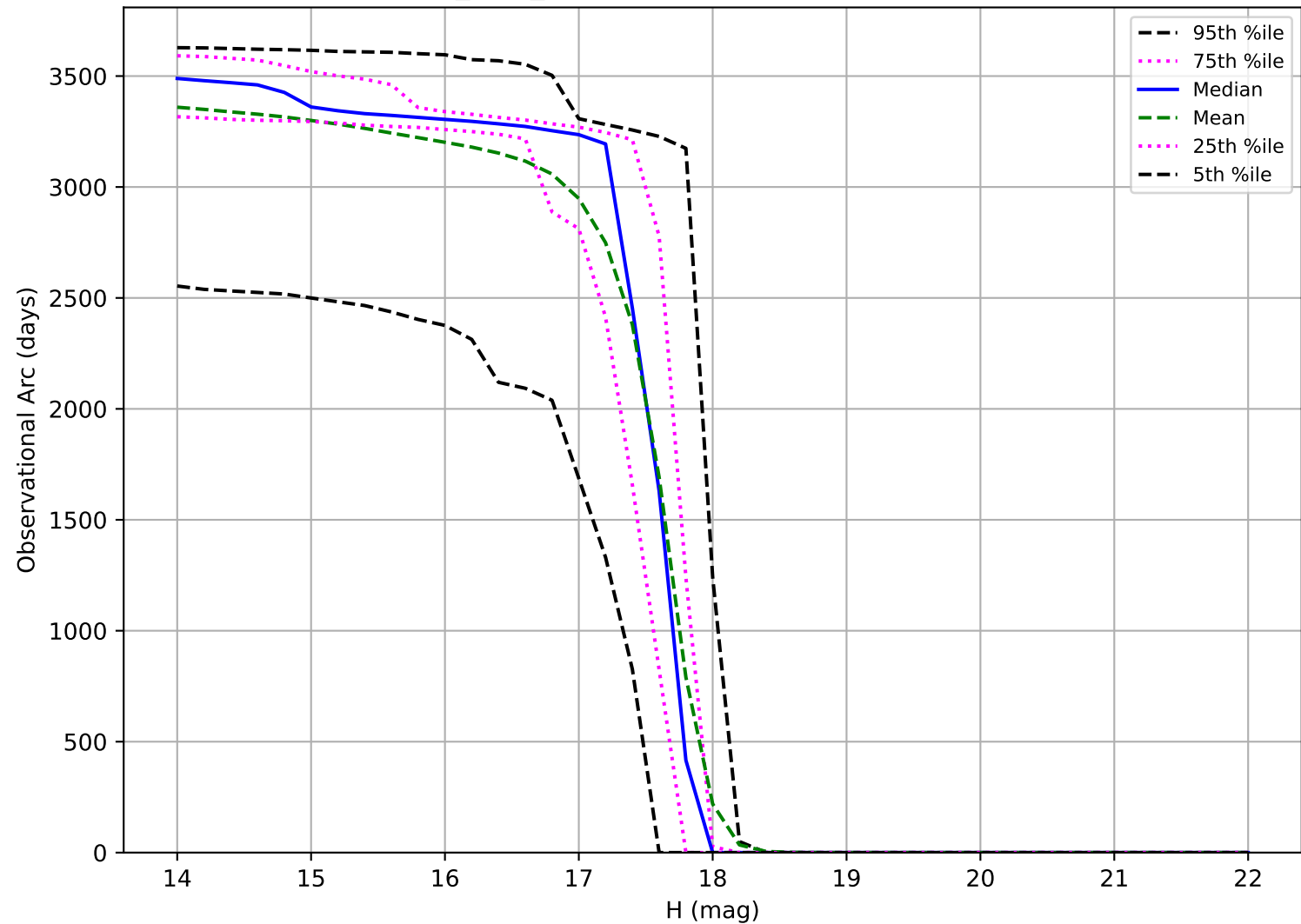
baseline_v3.4_10yrs: Observational Arc Length Trojan
