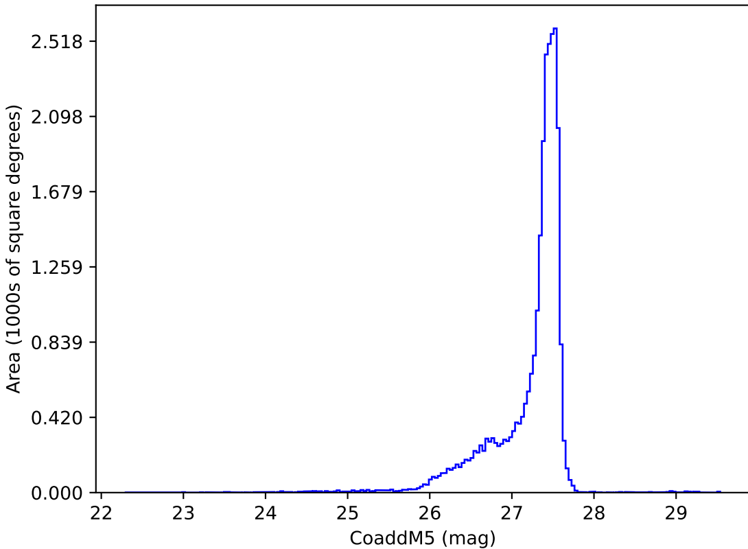
baseline_v3.5_10yrs : CoaddM5
