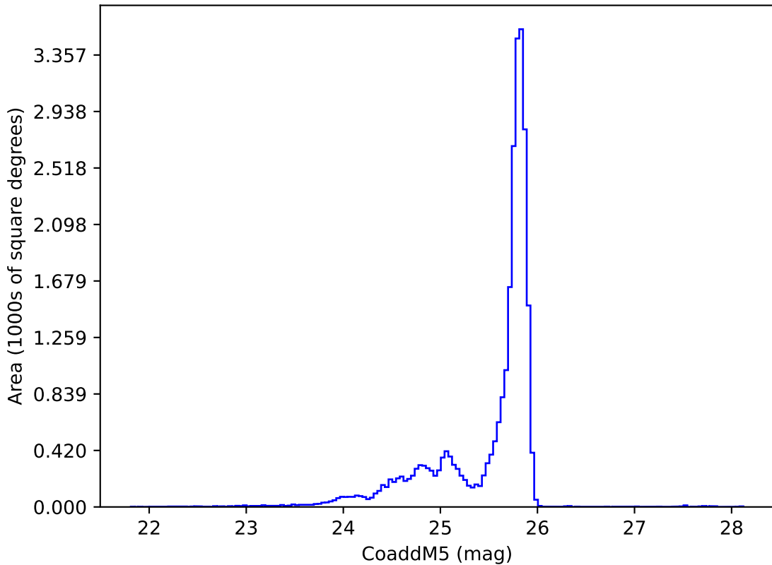
baseline_v3.5_10yrs z: CoaddM5
