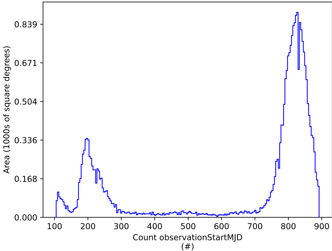
baseline_v3.5_10yrs : Count observationStartMJD
