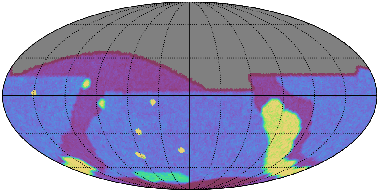
baseline_v3.5_10yrs g: Count observationStartMJD
