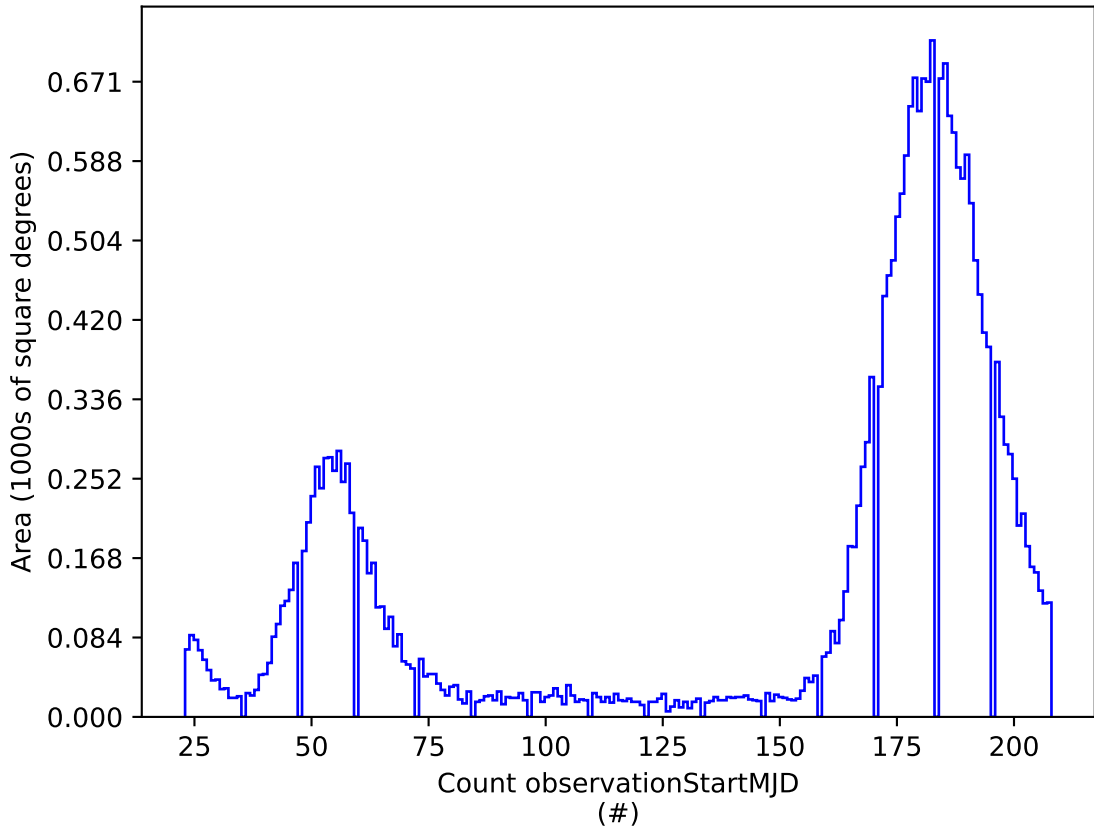
baseline_v3.5_10yrs r: Count observationStartMJD
