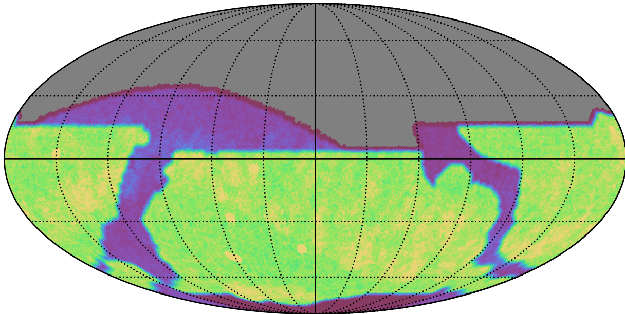
baseline_v3.5_10yrs r: Count observationStartMJD
