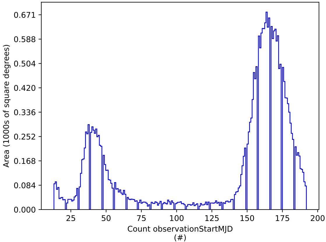
baseline_v3.5_10yrs z: Count observationStartMJD
