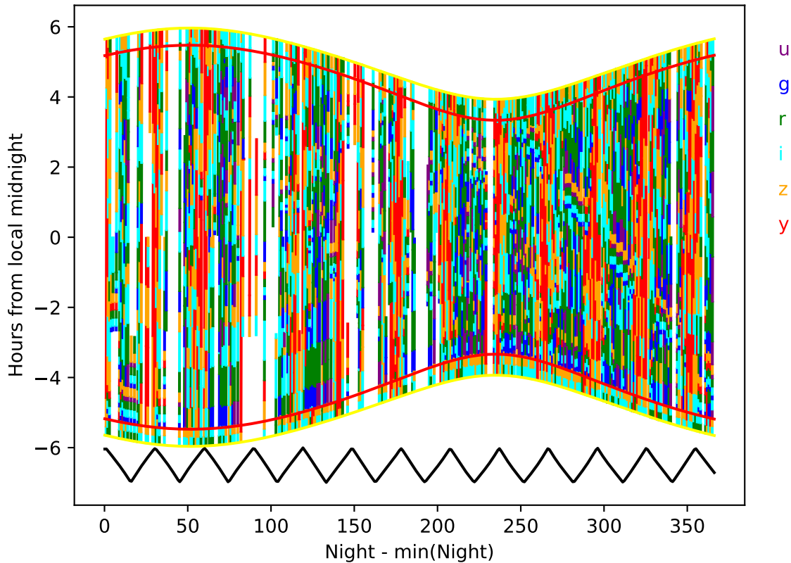
baseline_v3.5_10yrs year 1-2: Hourglass
