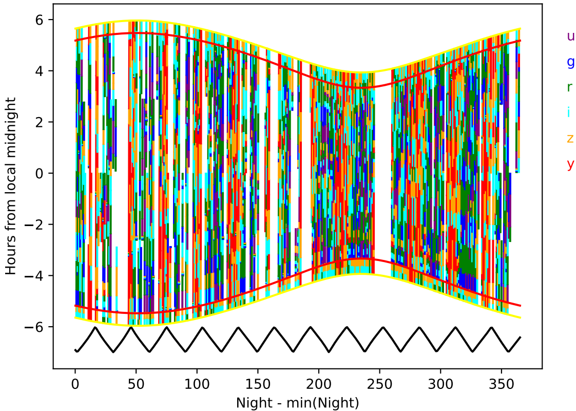
baseline_v3.5_10yrs year 5-6: Hourglass
