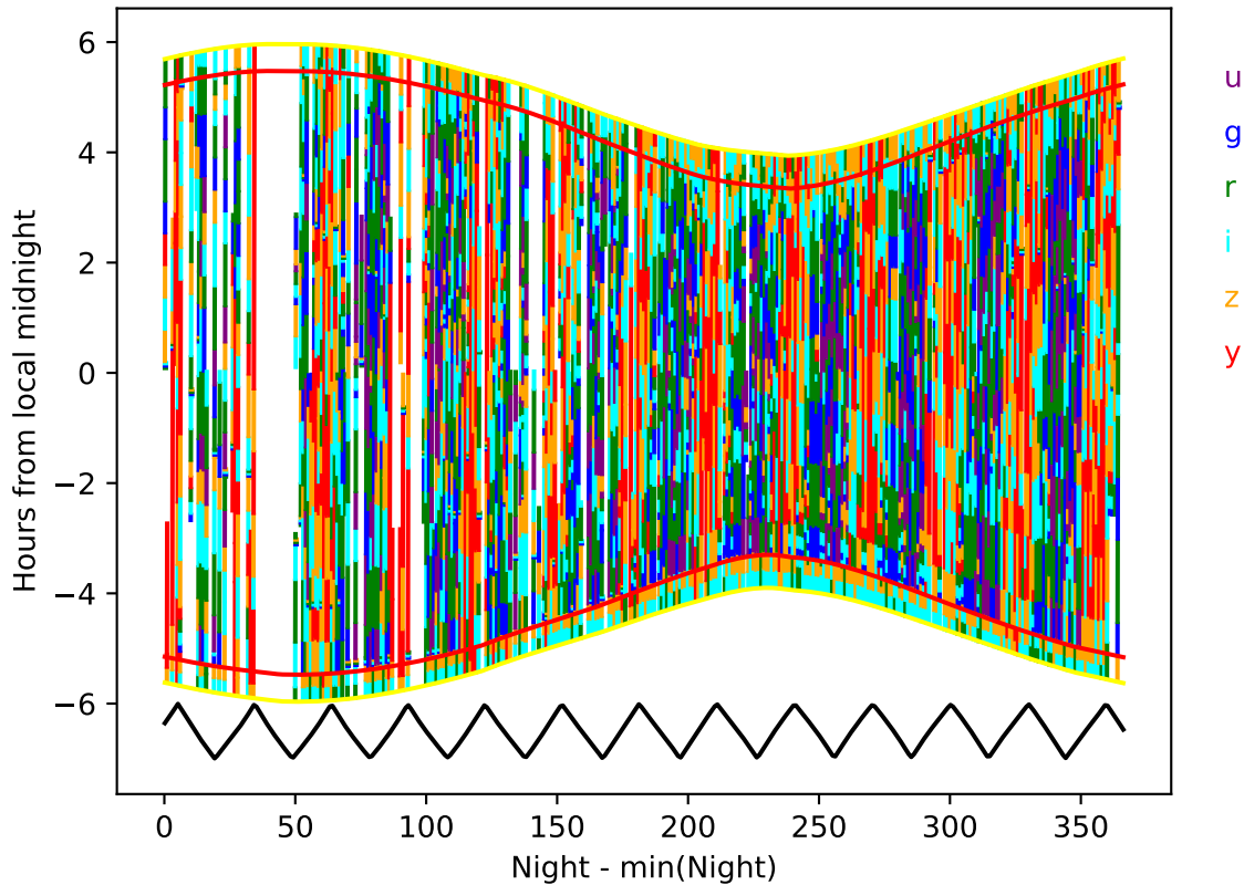
baseline_v3.5_10yrs year 6-7: Hourglass
