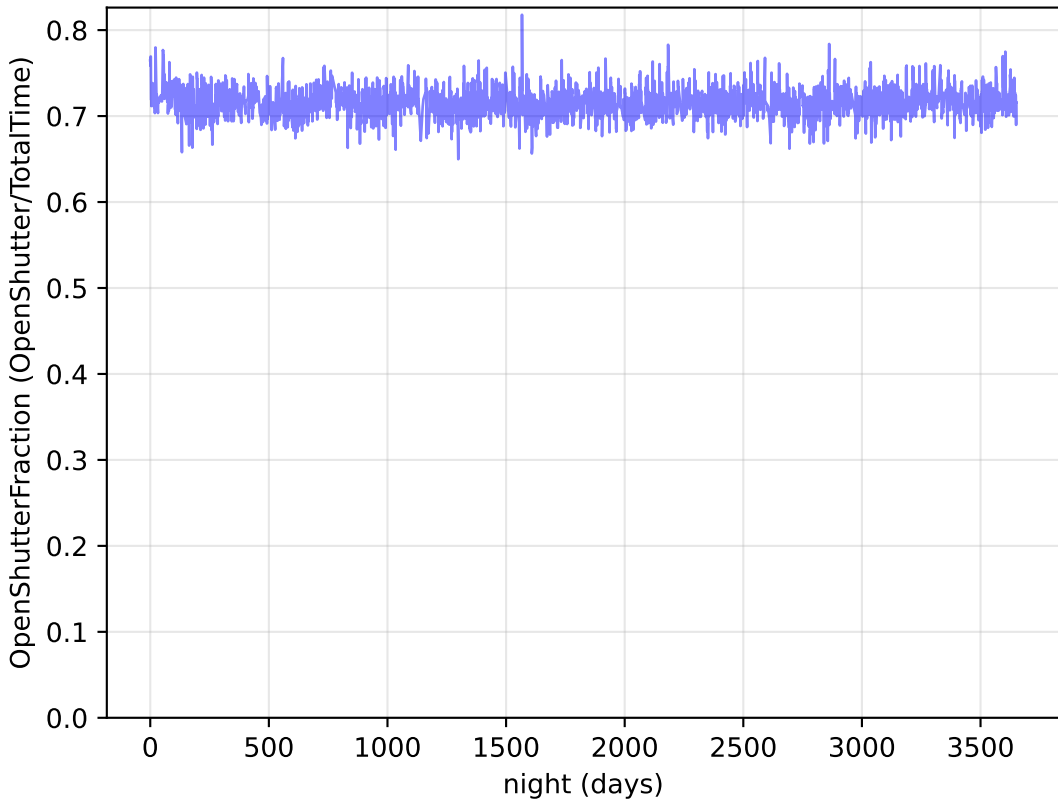
baseline_v3.5_10yrs : OpenShutterFraction
