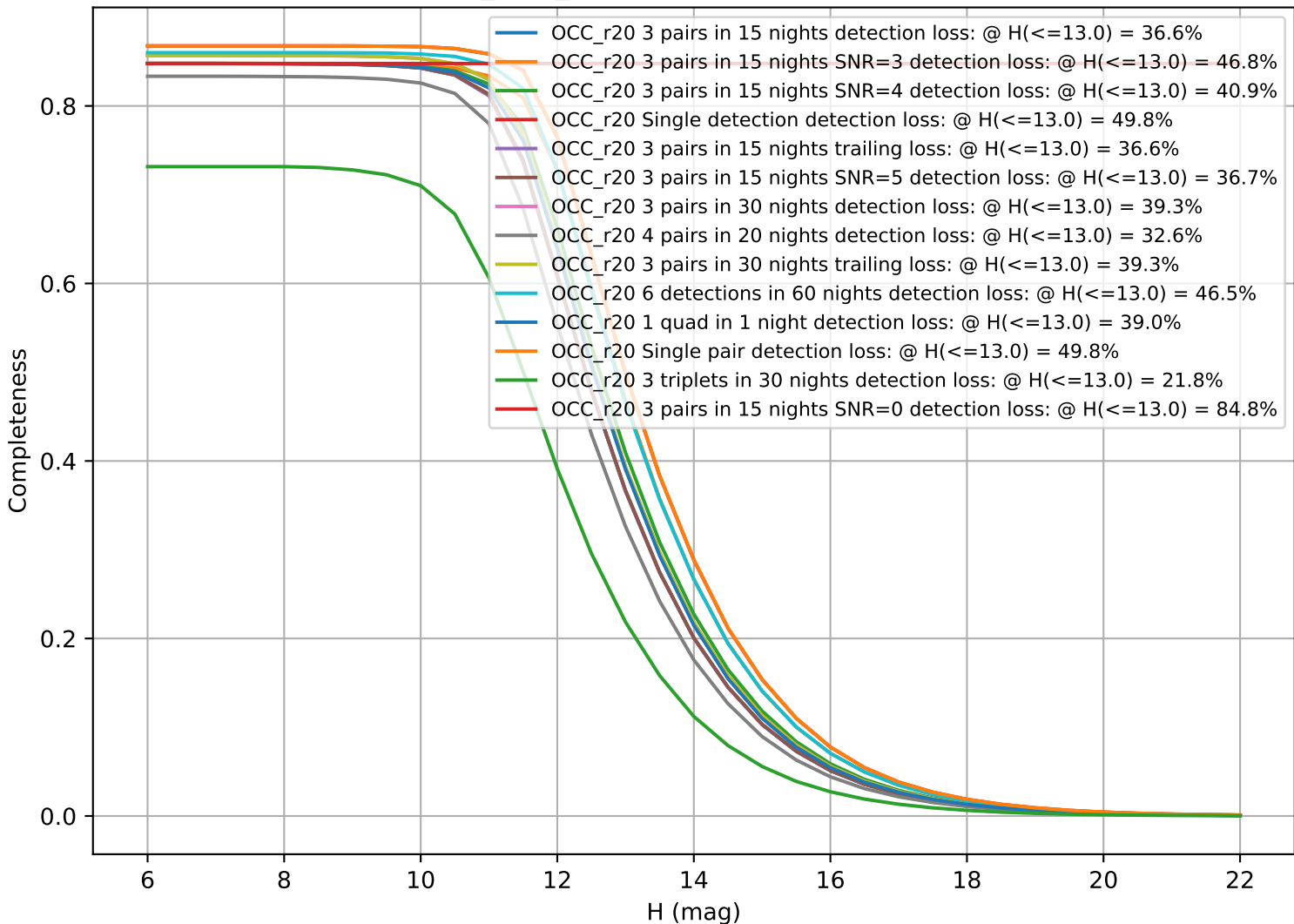
baseline_v3.5_10yrs: CumulativeCompleteness
