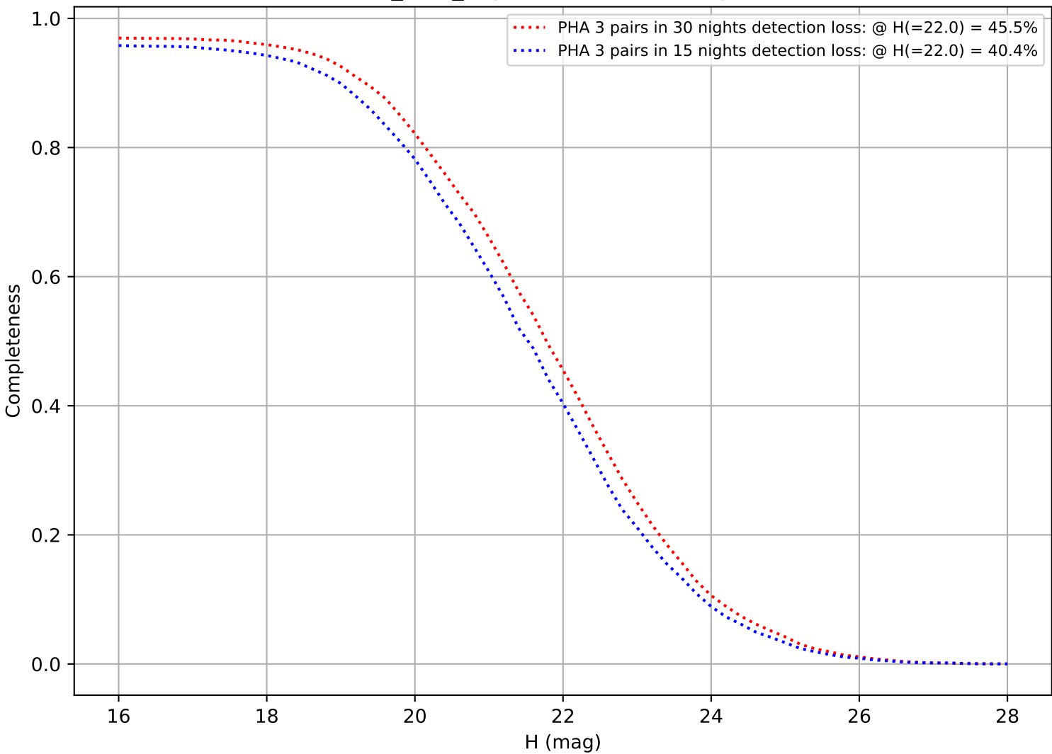
baseline_v3.5_10yrs: DifferentialCompleteness
