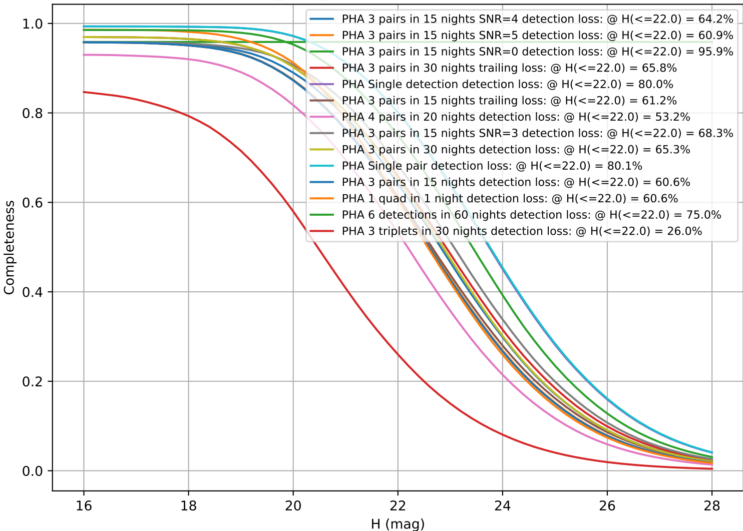
baseline_v3.5_10yrs: CumulativeCompleteness
