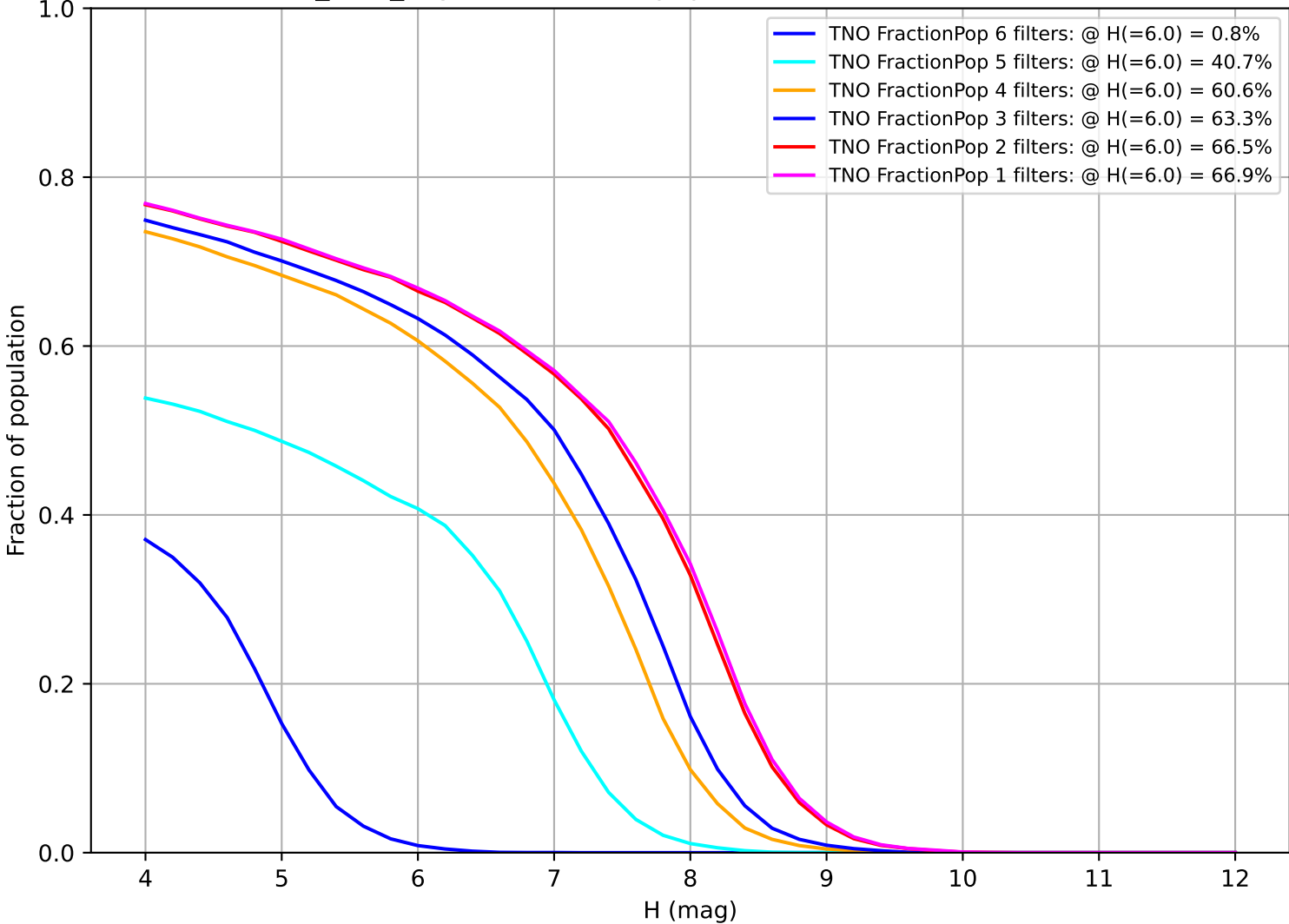
baseline_v3.5_10yrs: Fraction of population with colors in X filters TNO
