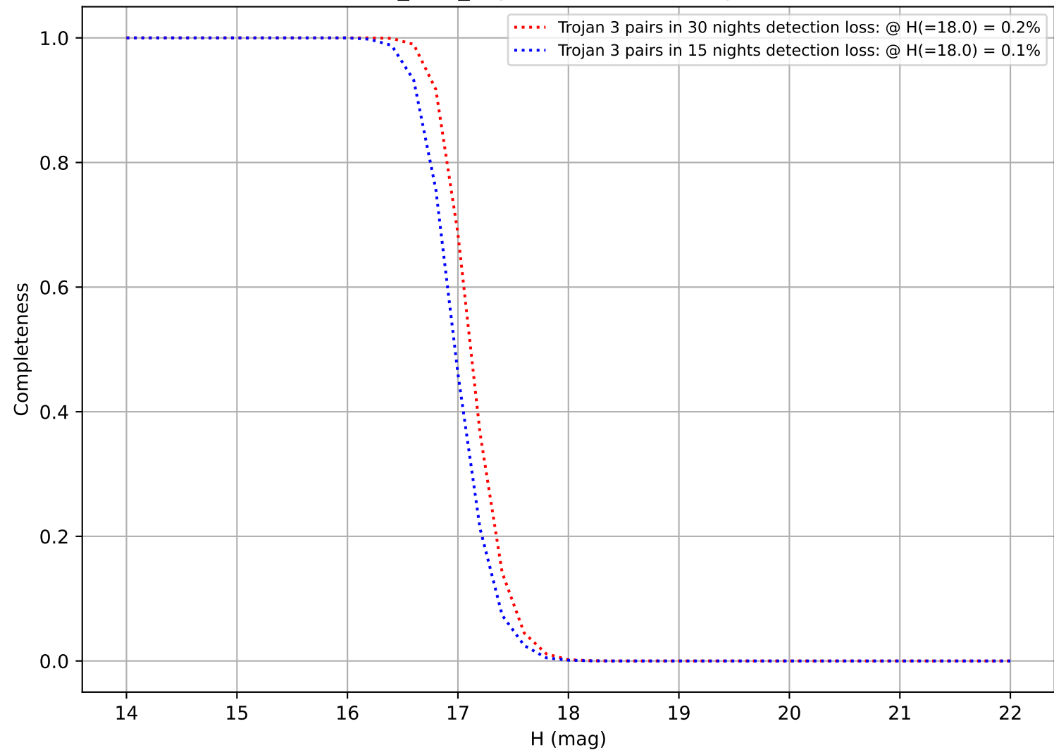
baseline_v3.5_10yrs: DifferentialCompleteness
