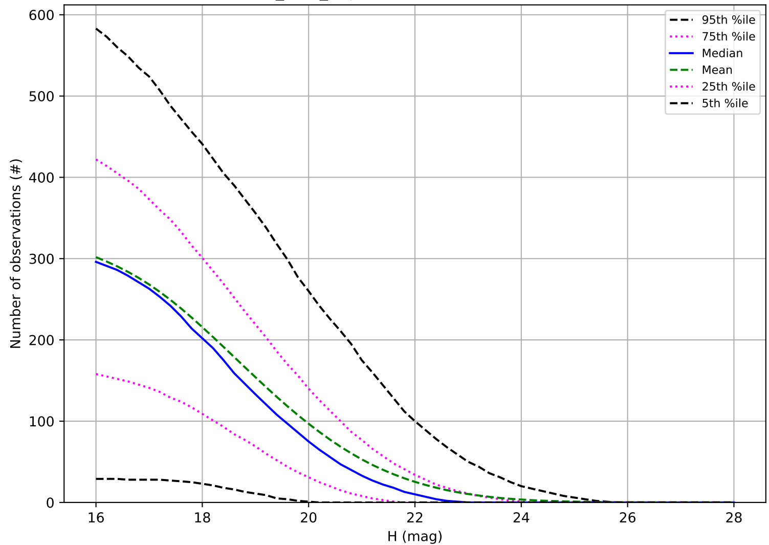
baseline_v3.5_10yrs: Number of observations NEO
