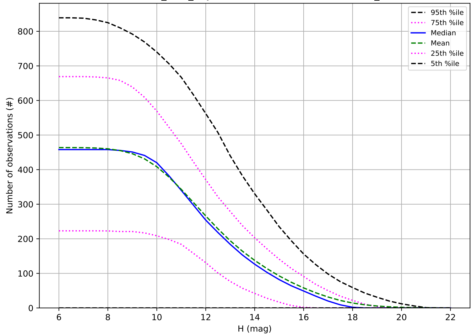
baseline_v3.5_10yrs: Number of observations OCC_r5
