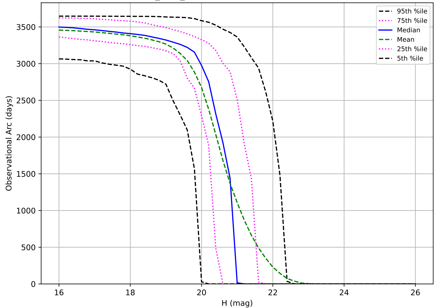
baseline_v3.5_10yrs: Observational Arc Length MBA
